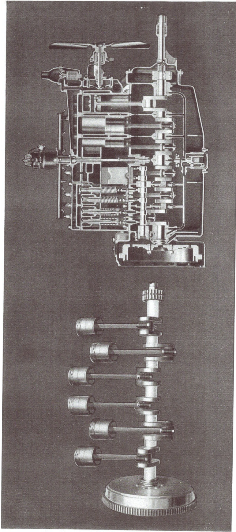
SINGLE-SIX CRANKSHAFT—Shows the seven main bearings and machined all over surfaces. Perfectly balanced and contributing greatly to freedom from motor vibration.
