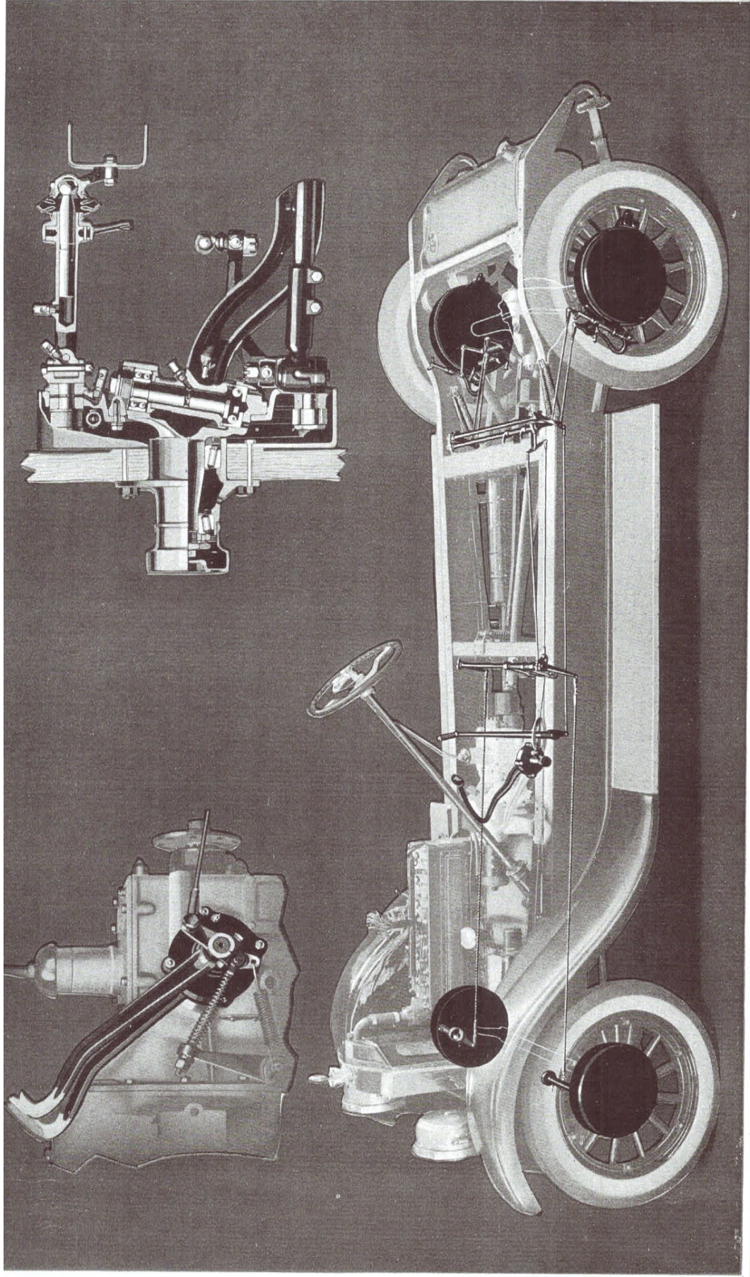
PLANETARY STEP-UP GEAR—Affords maximum braking pressure with minimum of pedal travel and effort.
