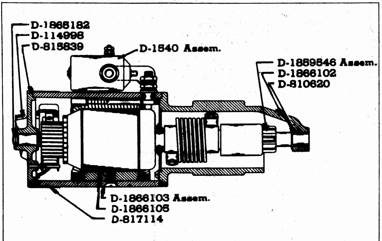
Models 1500-1-2
