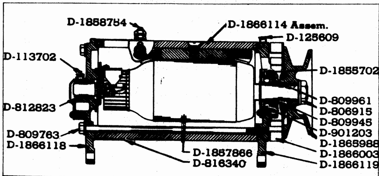
Models 1500-1-2
