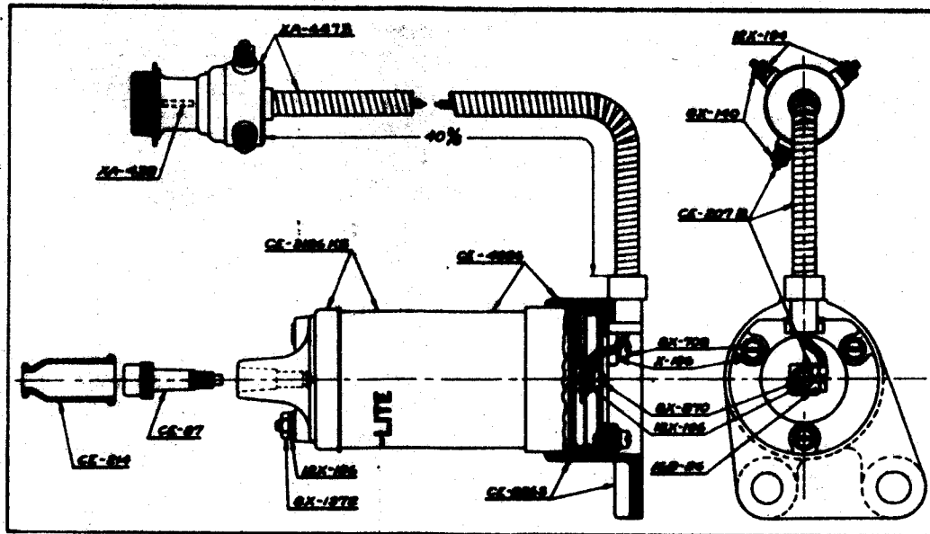
Models 1500-1-2 (6 Volt)
