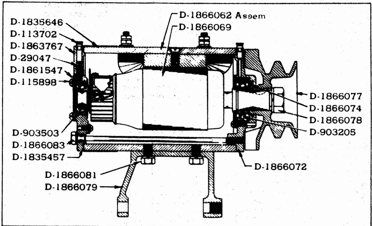
Model 1506-7-8
