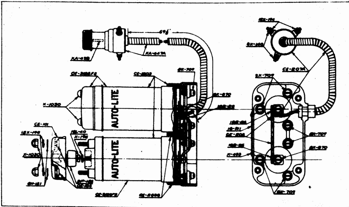
Models 1506-7-8 (6 Volt)
