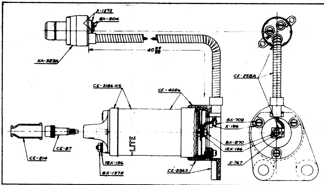
Models 1603-4-5 (6 Volt)
