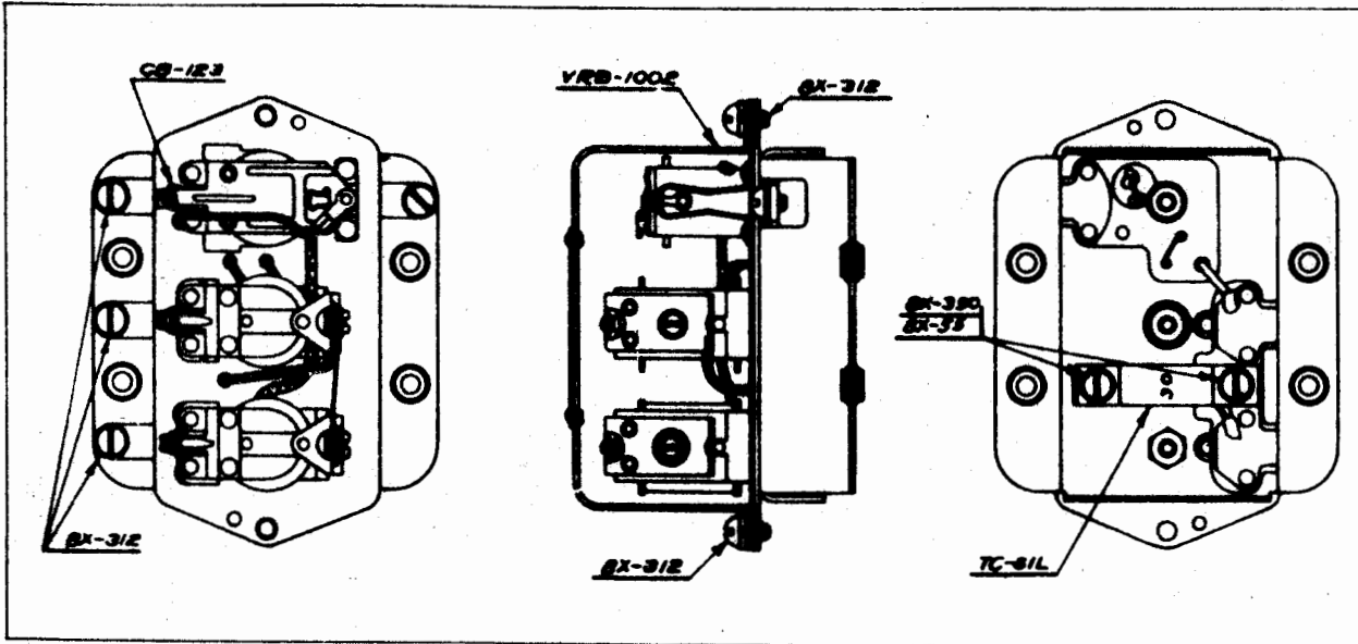
Models 1500-1-2, 1603-4-5 (6 Volt)
