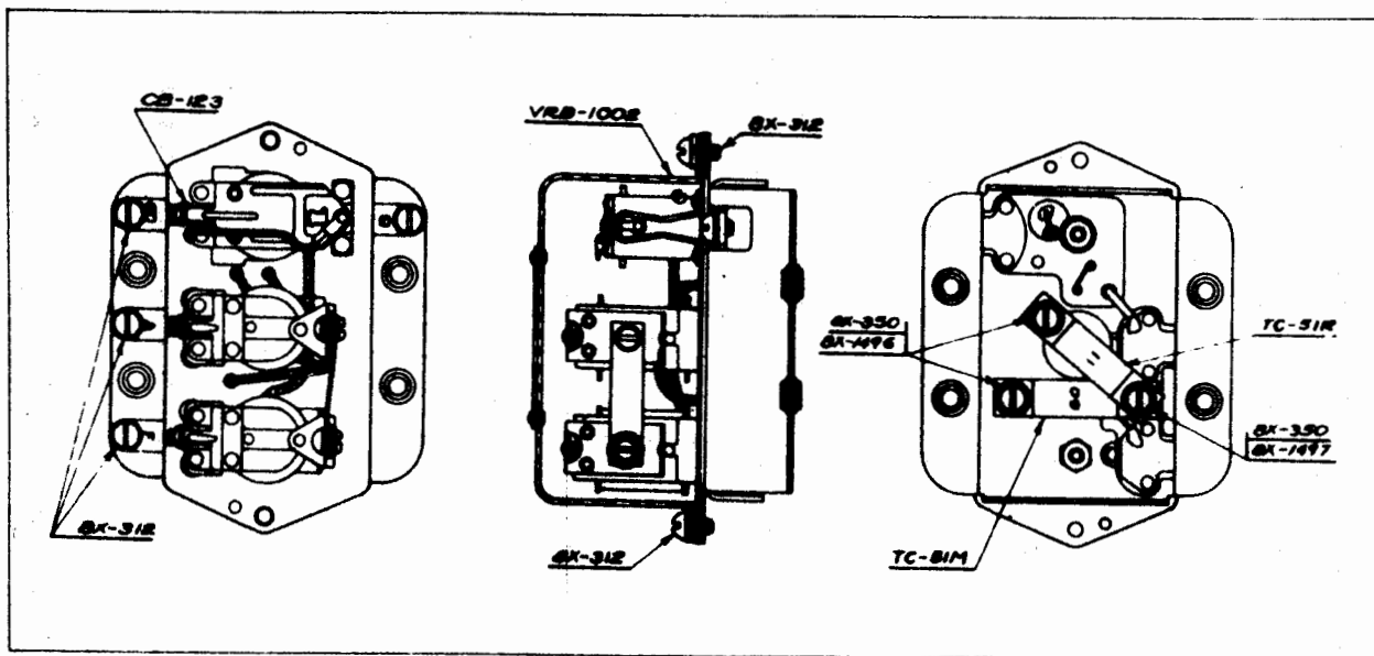
Models 1506-7-8, 1607-8, 1707-8 (6 Volt)
