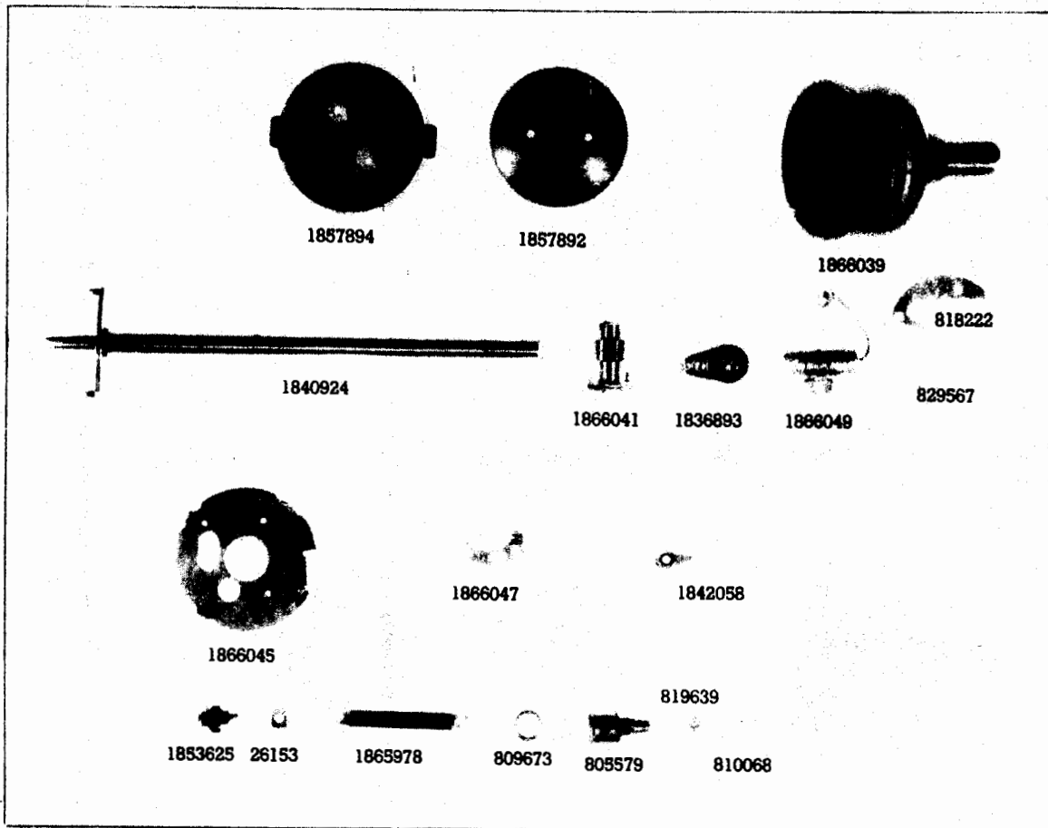
Models 1500-1-2
